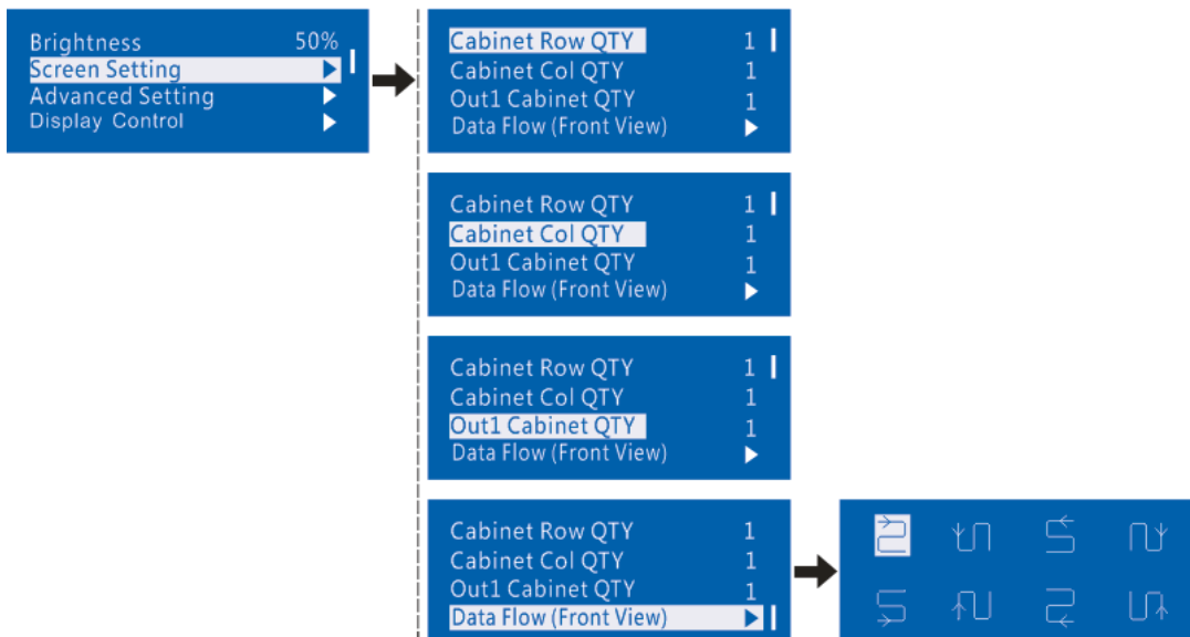
Figure 6-1 Quick configuration
