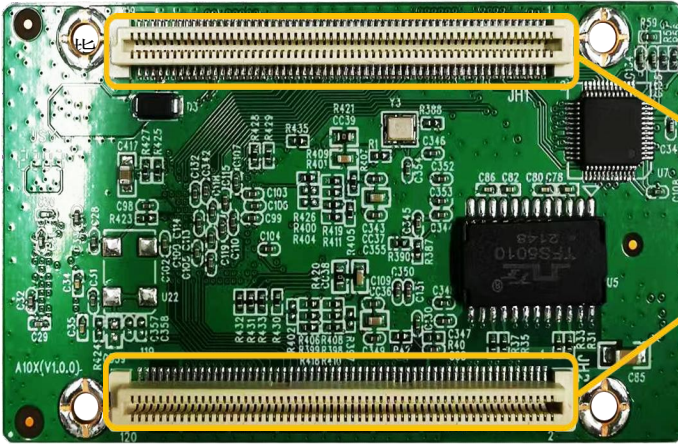
High Precision Connector
